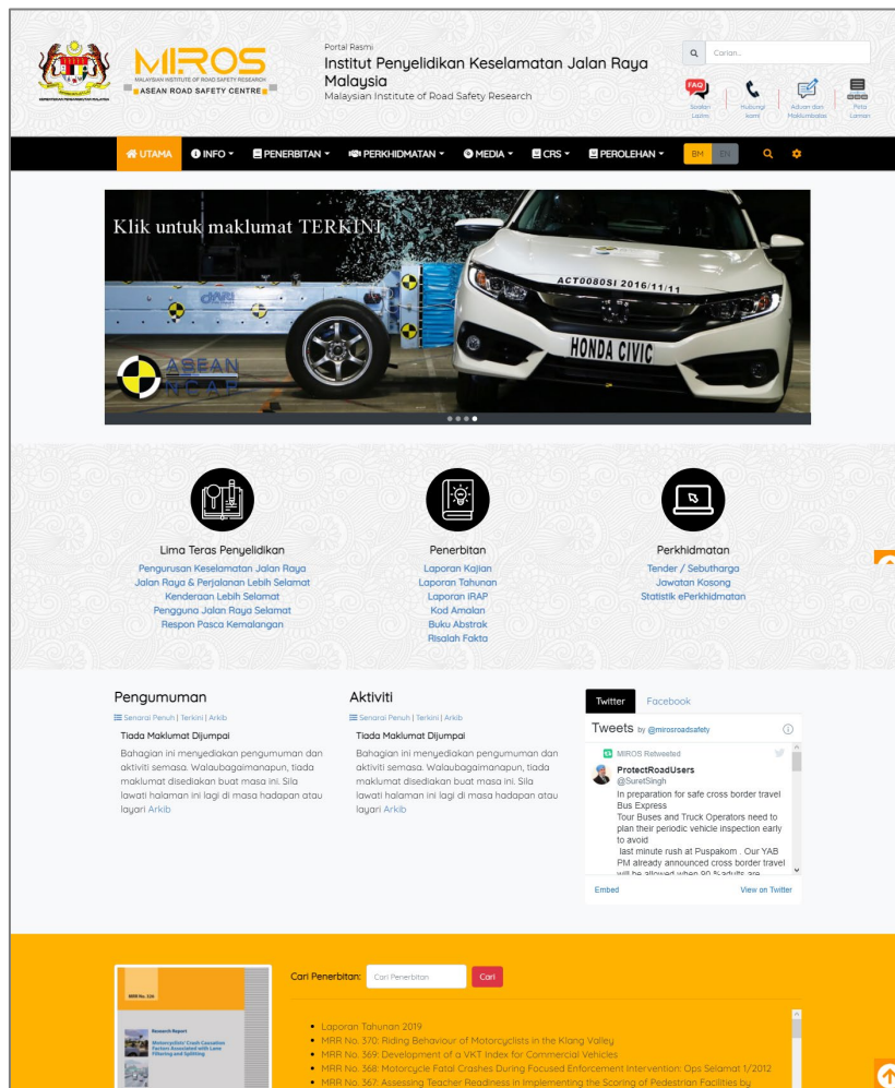
Desktop view
